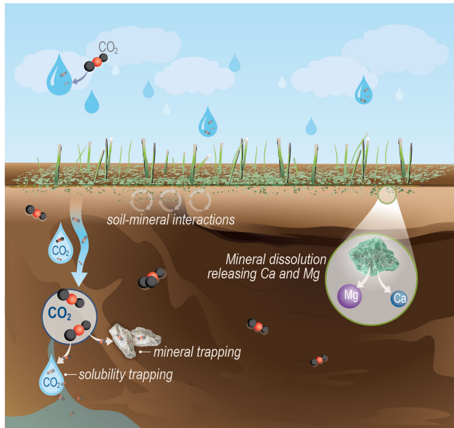
Figure 1: Chemical weathering in soil [7]
